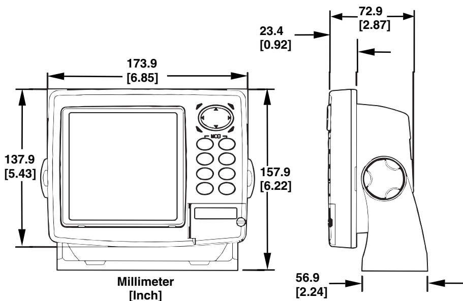
Front view (left) and side view (right) showing dimensions of the IntelliMap 502C when mounted on gimbal bracket.
